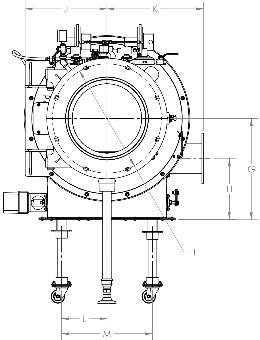
ADVANCED PERFORMANCE INJECT-AIRE AXIAL FAN BURNER DIMENSIONS, GIVEN IN INCHES
